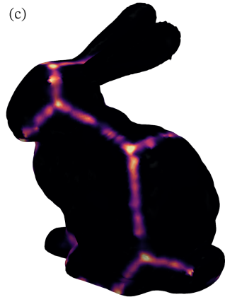
Chart entropy
