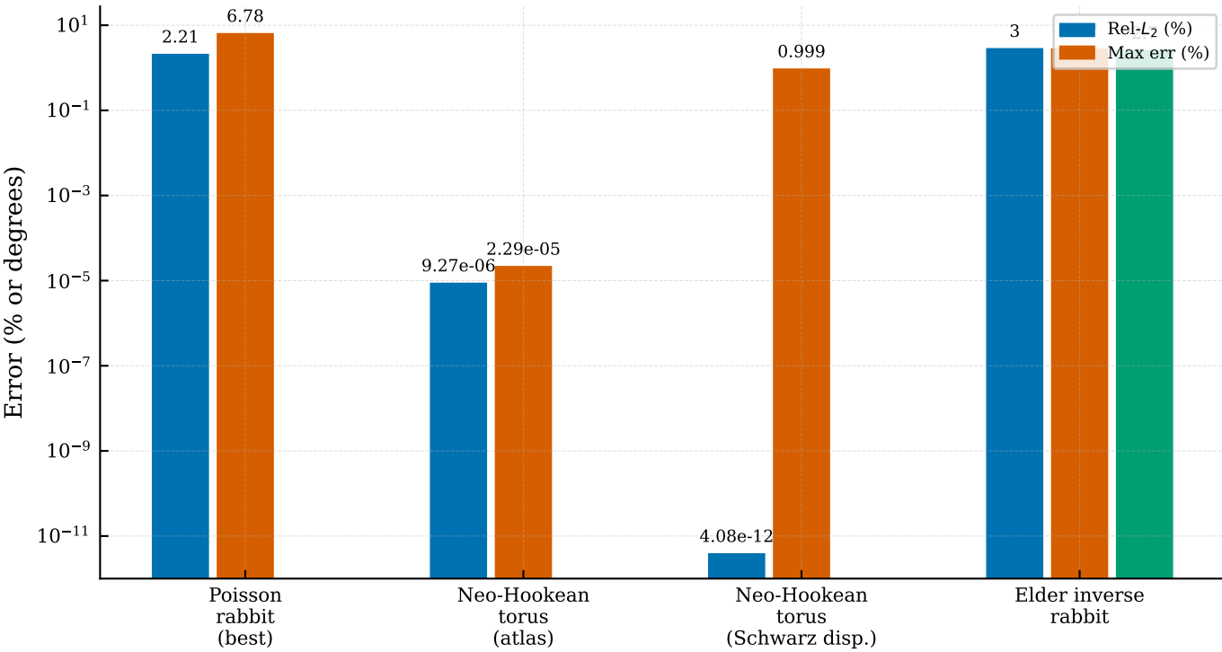
Benchmark summary — all numerical examples
