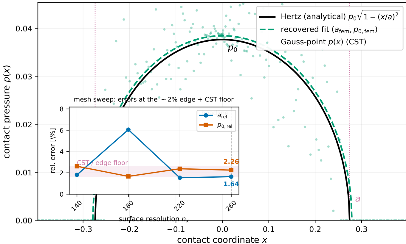
CV-8 deformable Hertz: recovered pressure vs. analytical half-ellipse ( E^* = 0.549 , R = 2.0 , finest mesh n_x = 260 )
