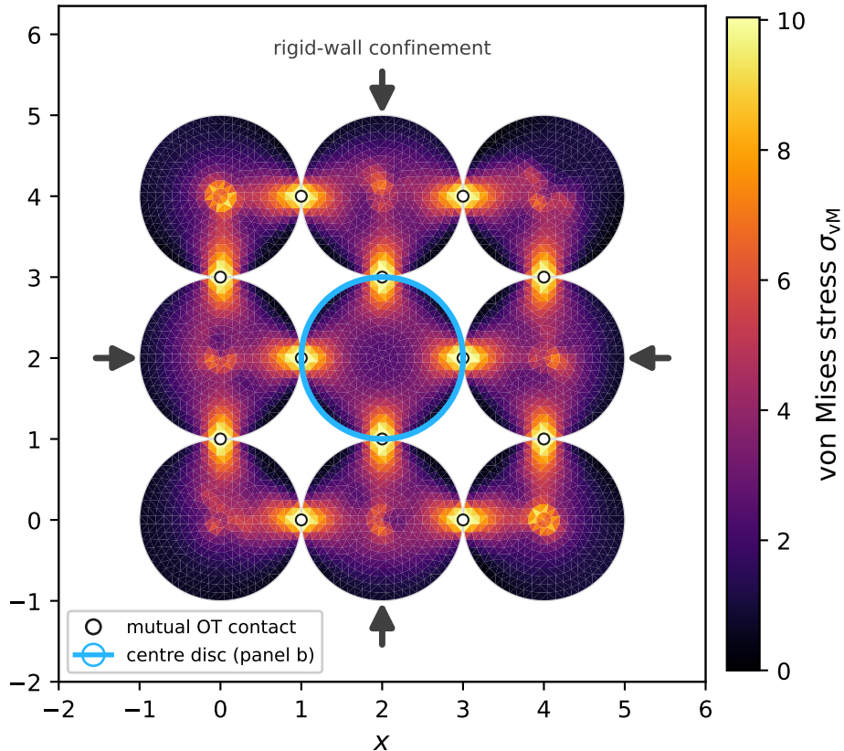
(a) 3 \times 3 elastic discs, 12 mutual OT contacts
