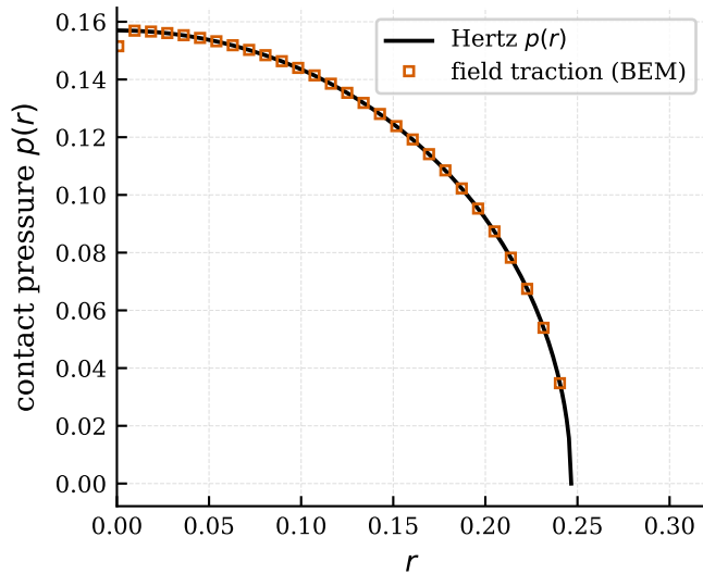
(b) CV-1c 3-D axisymmetric Hertz
