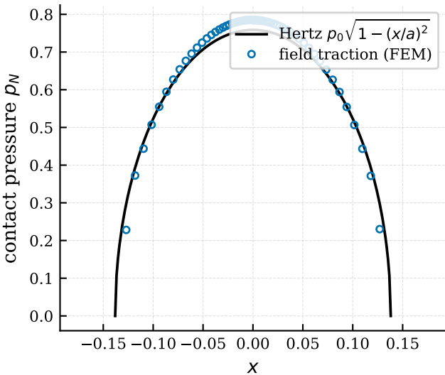
(a) CV-1b 2-D line Hertz
