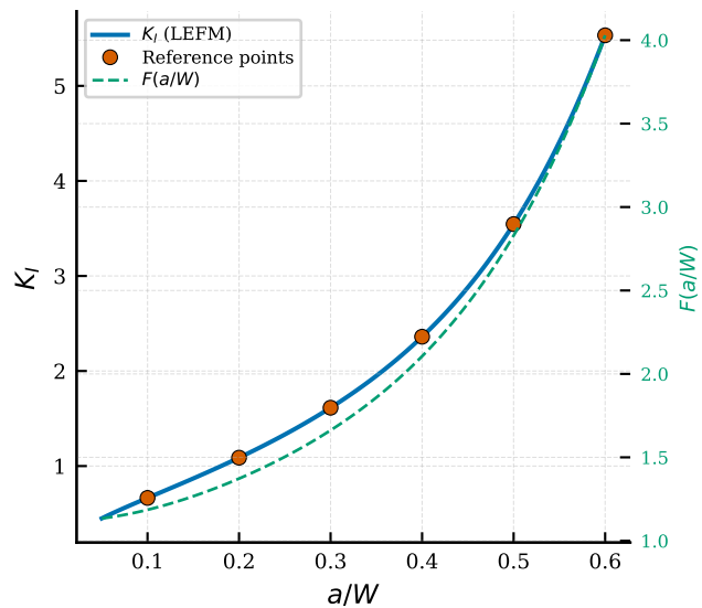
(b) Stress intensity factor
