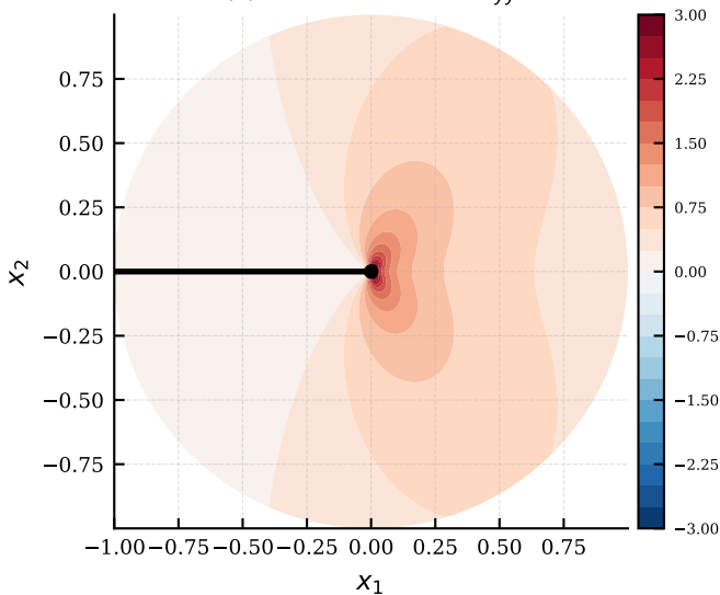
(c) Williams stress \sigma_{yy}
