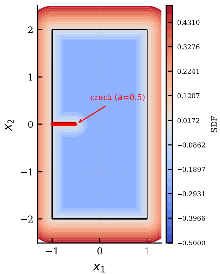
(e) Cracked plate SDF ( x_3=0 )
