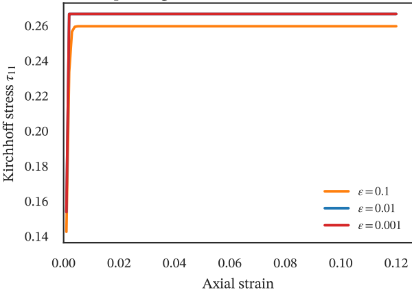
(a) Softplus regularisation ( \varepsilon effect)
