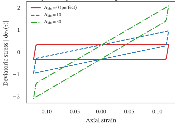
(b) Cyclic response (Bauschinger effect)
