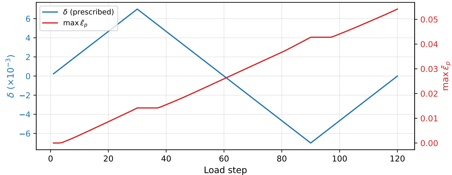
Loading history and plastic strain accumulation ( n_{\text{cells}} = 6 )
