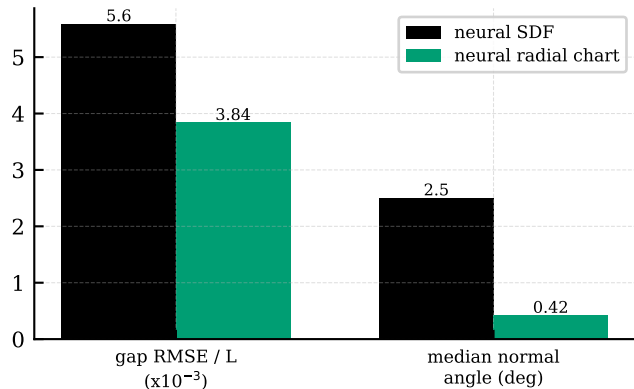
CV-5: transition-map chart beats the SDF (cusped superformula)
