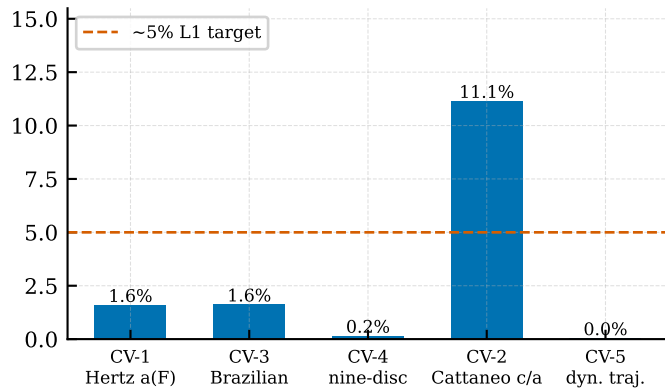
L1 mechanics: numerical vs closed form
