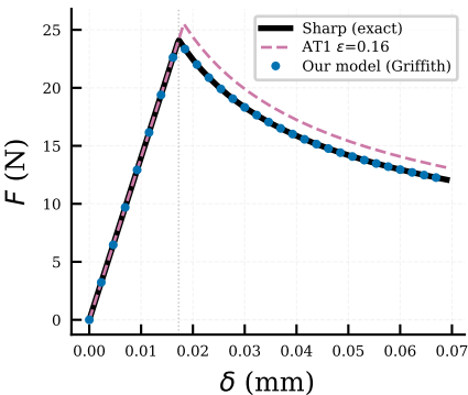
(a) Force-displacement
