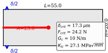
(c) DCB schematic
