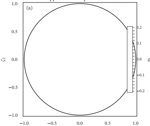
Mapped domain: absolute error
