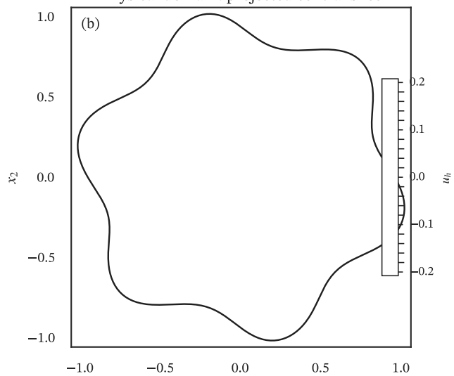
Physical domain: projected error
