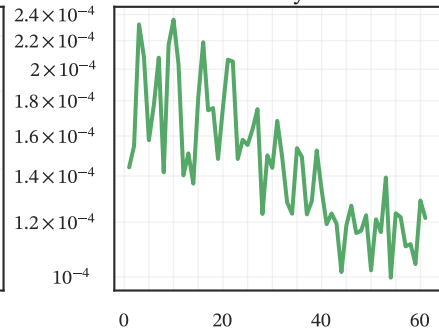
Boundary loss
