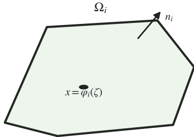
Normal map
