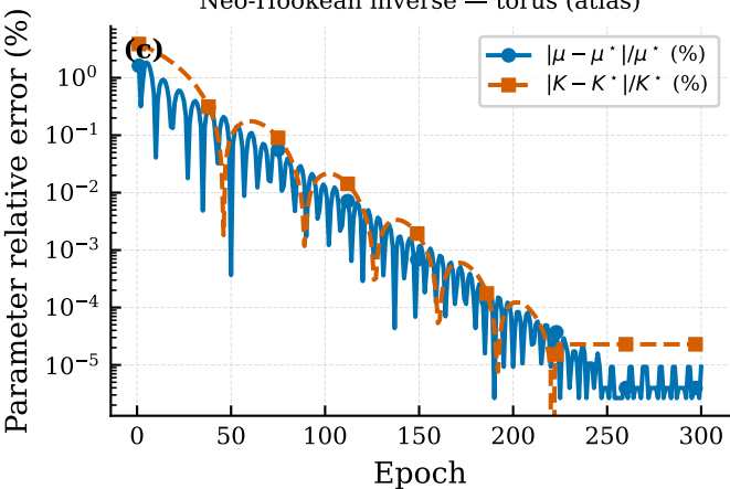
Neo-Hookean inverse — torus (atlas)
