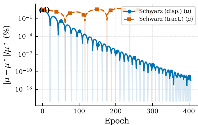
Neo-Hookean inverse — torus (Schwarz)
