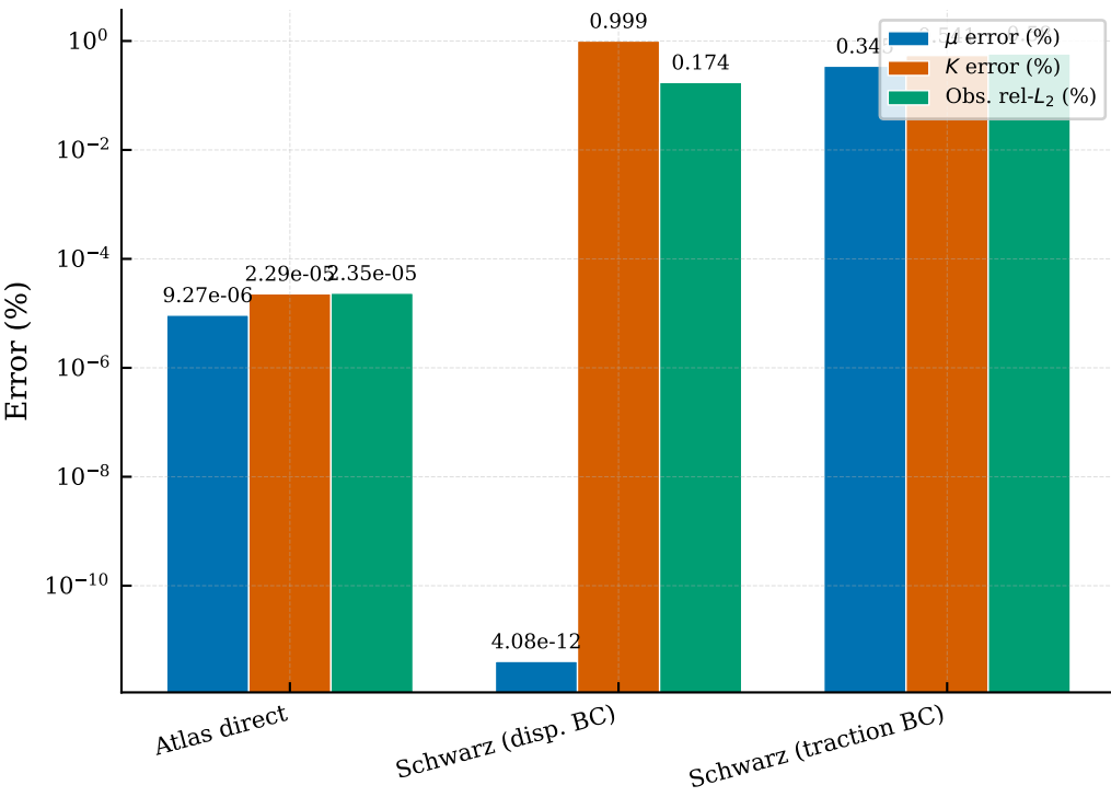
Inverse neo-Hookean on torus — final parameter errors
