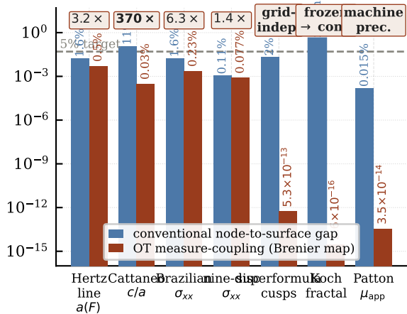
(a) conventional gap vs. OT coupling
