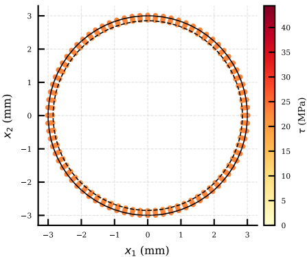
(a) \tau at mid-section (step 33)
