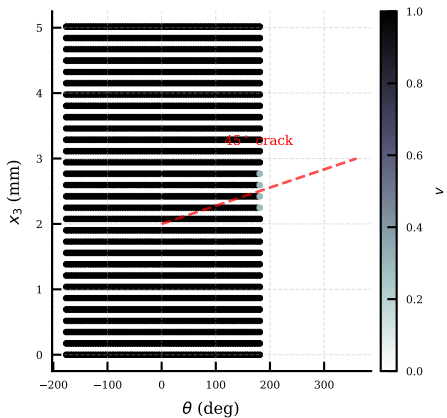
(b) Phase field v (unwrapped)
