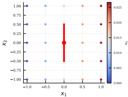
(e) Task 5: u_x + crack + 3 spawned pairs
