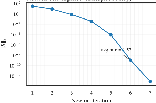
Newton convergence (elastoplastic step)
