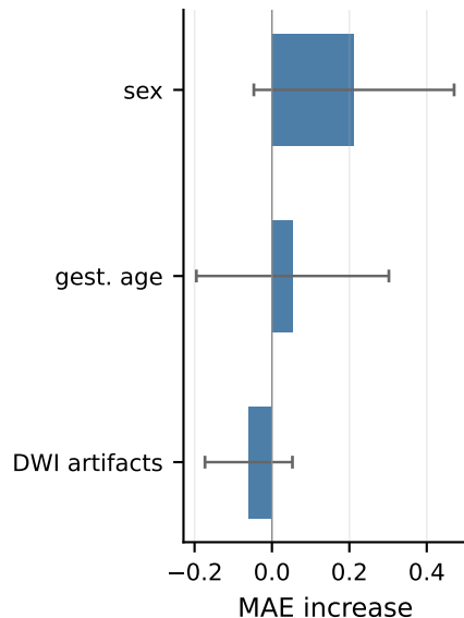
Covariates
