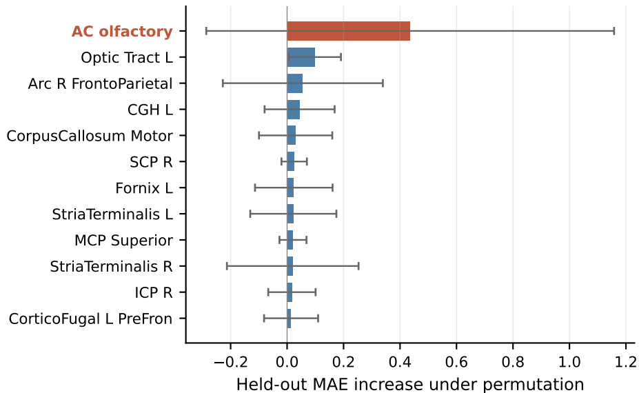
Top 12 tracts by OOF permutation importance
