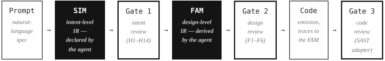
Figure 1. The generation pipeline with two intermediate representations and three deterministic gates. The SIM (intent level) is checked for the promises; the FAM (design level) for the arithmetic; the code (implementation level) for the defects that can be found only at the code level. The agent appears at the two IR stages, which it authors; everything to their right — the three gates — is deterministic and inspectable.
