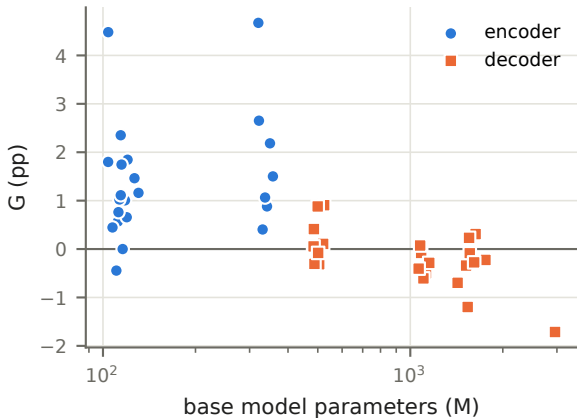
Extra rank and epochs: trained baseline – pool member
