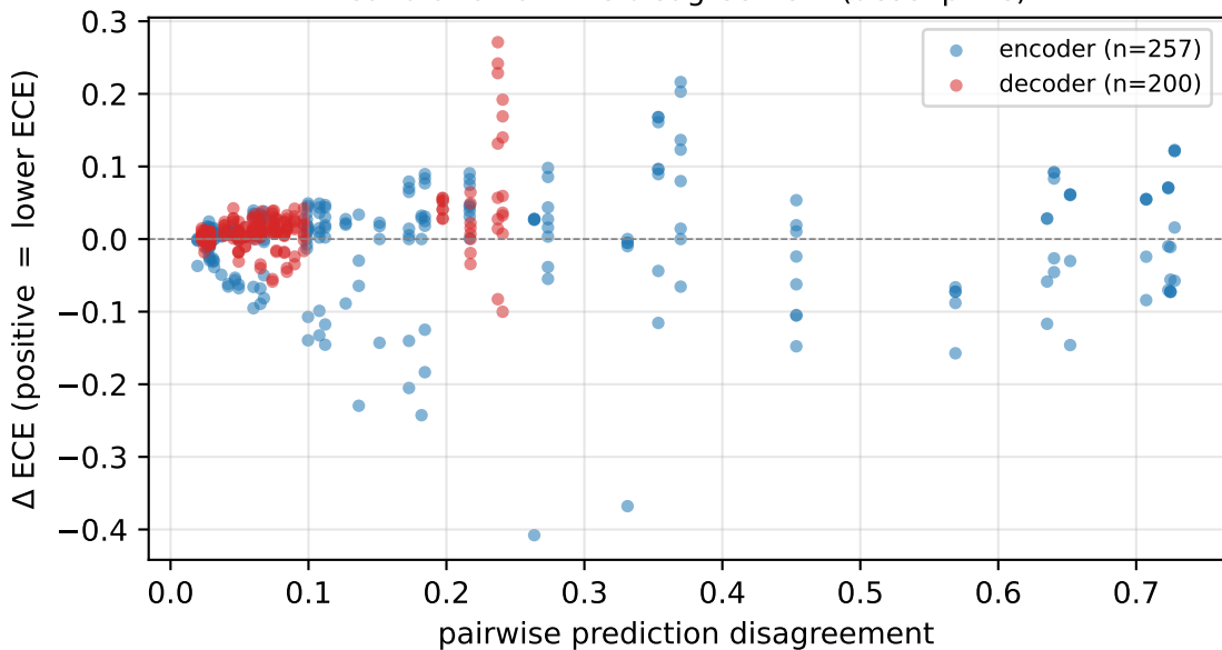
Calibration arm vs disagreement (descriptive)
