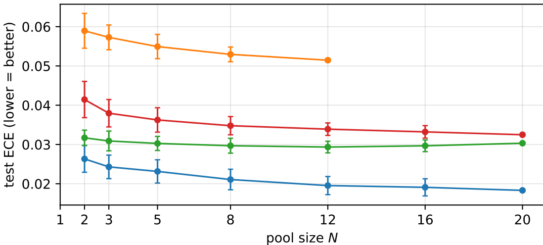
ECE vs. pool size N (modest decline continues to N=20 )
