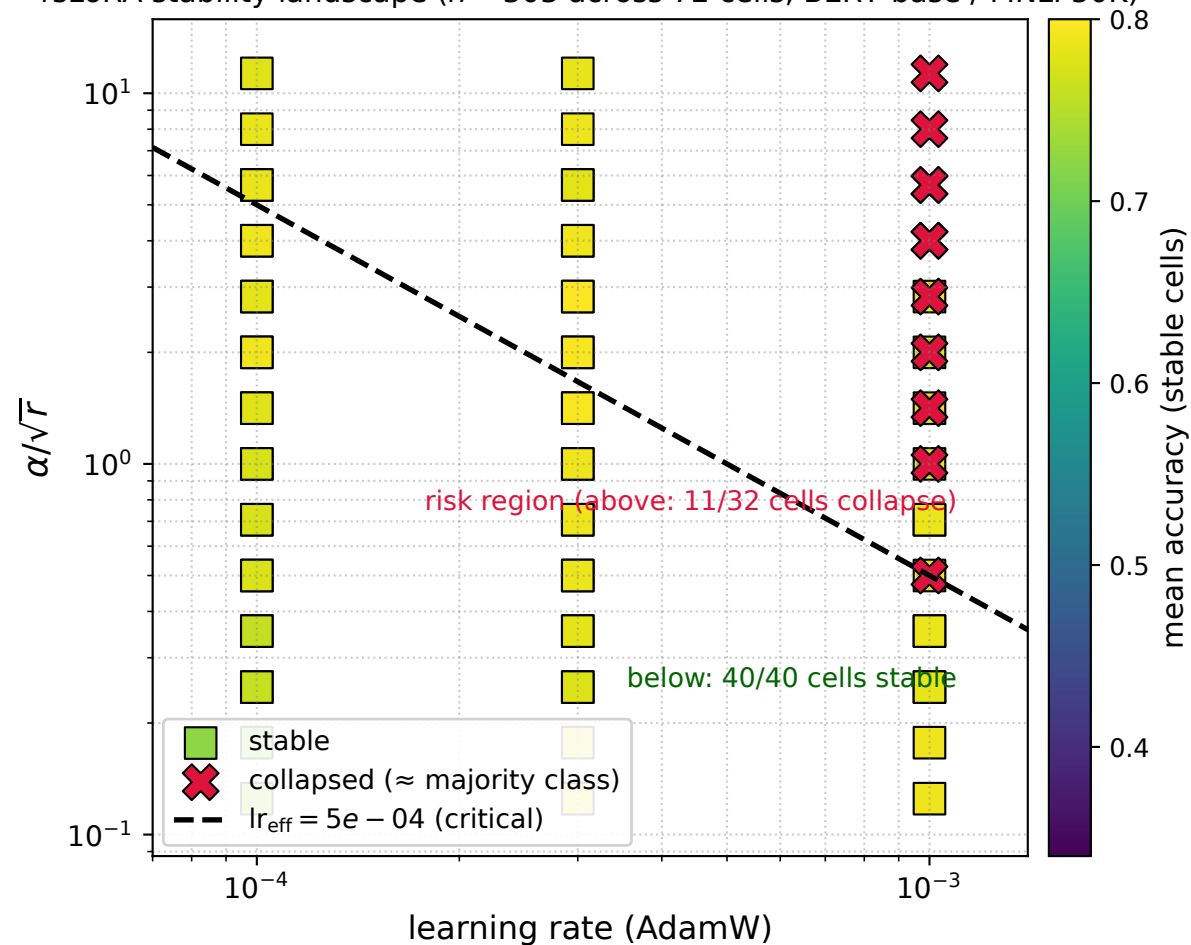
rsLoRA stability landscape ( n = 303 across 72 cells, BERT-base / MNLI 50K)
