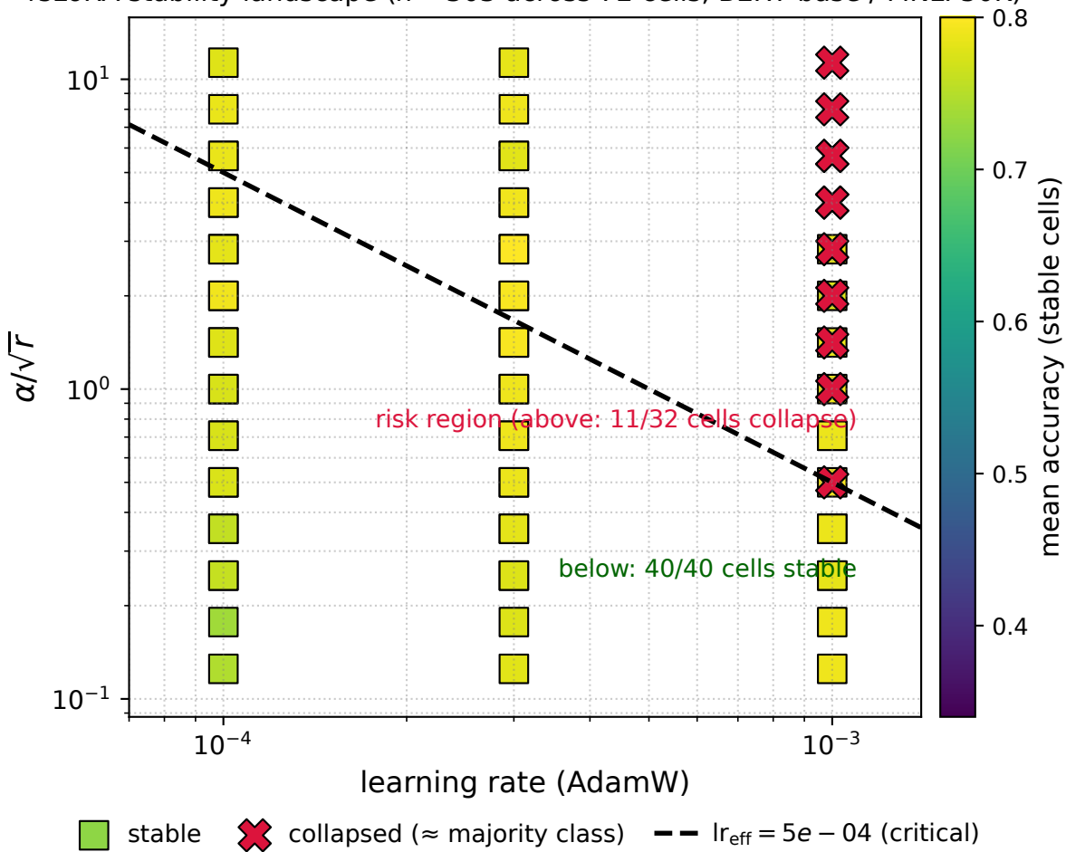
rsLoRA stability landscape ( n = 303 across 72 cells, BERT-base / MNLI 50K)
