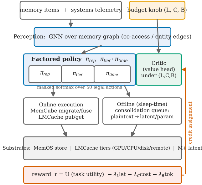
Fig. 1. The STOA control plane. A GNN perceives the memory graph; a factored, masking-exact policy and a budget-conditioned critic emit one action per item; online and sleep-time branches execute against the underlying store, tiers, and latent path. Task-utility reward flows back through credit assignment.
