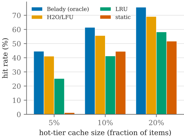
Tier-axis eviction ablation (RQ1)
