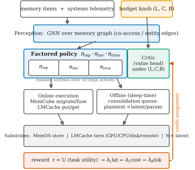
Figure 1: The STOA control plane. A GNN perceives the memory graph; a factored, masking-exact policy and a budget-conditioned critic emit one action per item; online and sleep-time branches execute against the underlying store, tiers, and latent path. Task-utility reward flows back through credit assignment.
