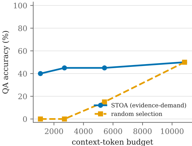
LoCoMo accuracy vs budget (LLM-judge)
