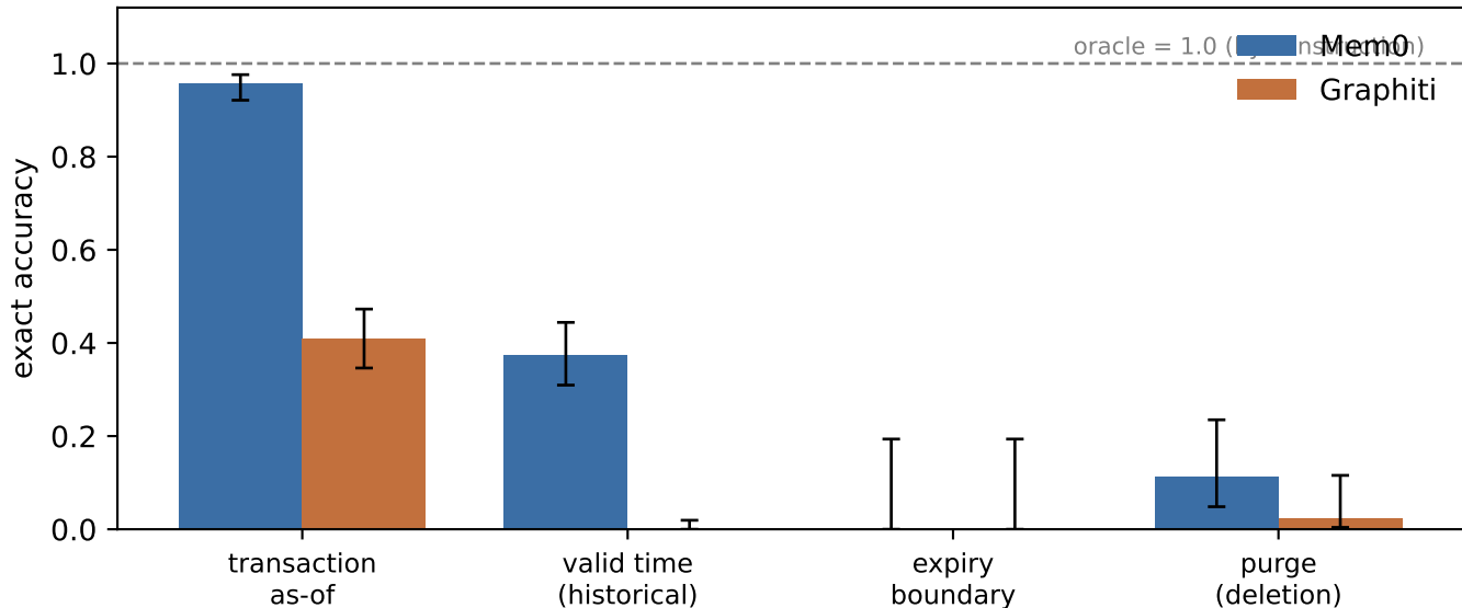
Per-category exact accuracy, 20 matched cells (Wilson 95% intervals)
