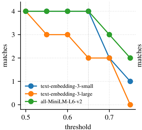
Primary R@10 (of 4)
