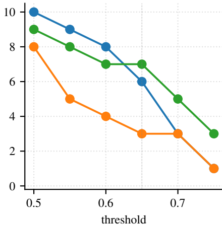
All-paradigm R@10 (of 10)
