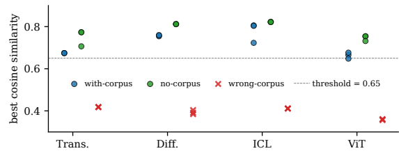
Figure 5: Per-paradigm best-cosine across 3 seeds (1, 2, 42) for the with-corpus (blue) and no-corpus (green) cells, plus all 4 wrong-corpus pairings (red x). The behavioural conclusions are seed-stable: no-corpus and wrong-corpus cells are identical R@10 across seeds; with-corpus drops the ViT cell of seed 42 just below the dashed 0.65 threshold (the 4/4/3 multi-seed bound in Limitations).
