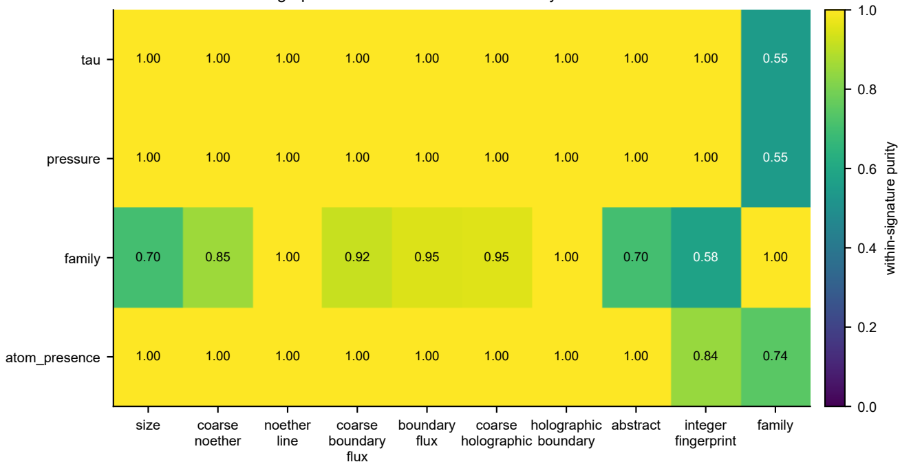
Holographic reconstruction: what boundary data determines
