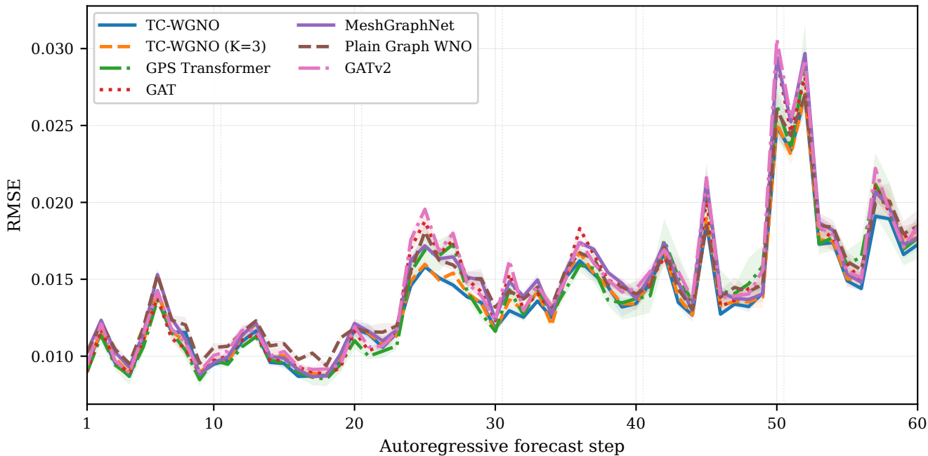
PFLOTRAN 60-step rollout
