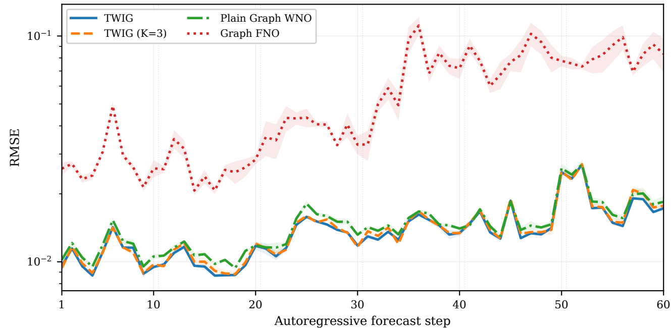
Graph neural operator comparison
