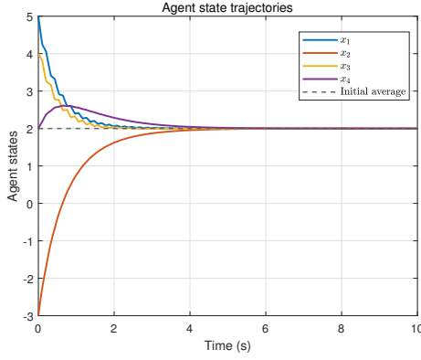
Fig. 2. Agent state trajectories under the proposed switching law.
