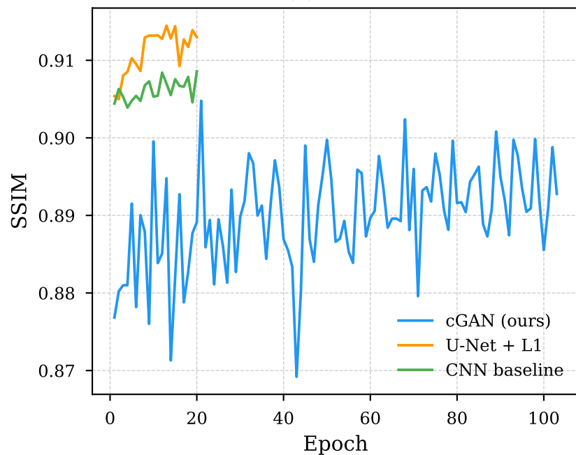
(c) SSIM
