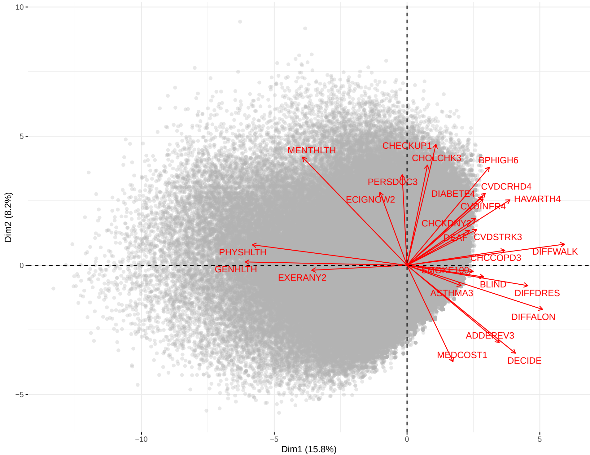
PCA Biplot (5000 sampled individuals)
