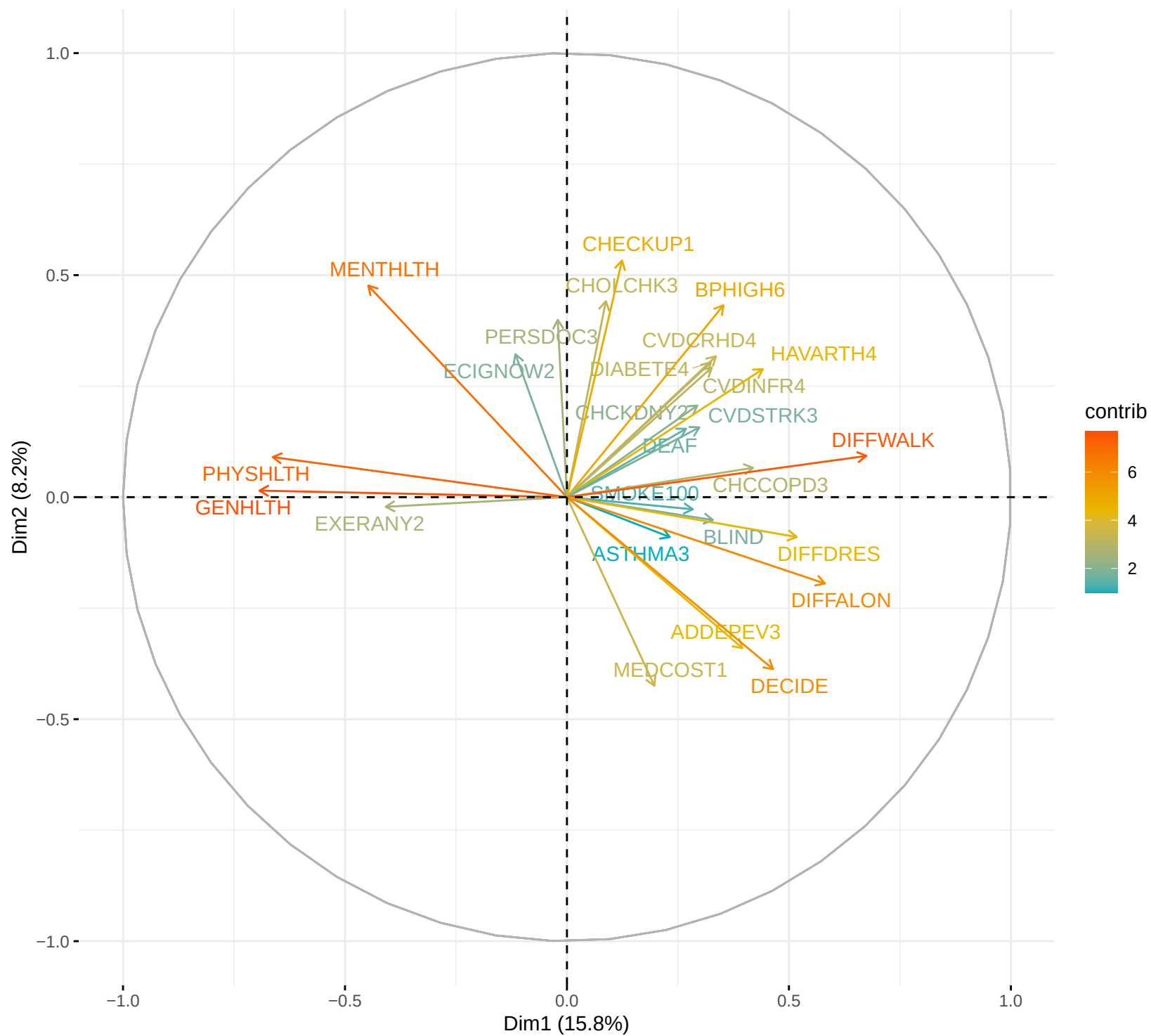
Variables – PCA (Dimensions 1–2)
