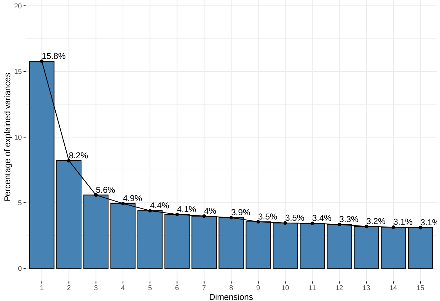
Scree Plot: Variance Explained by Components
