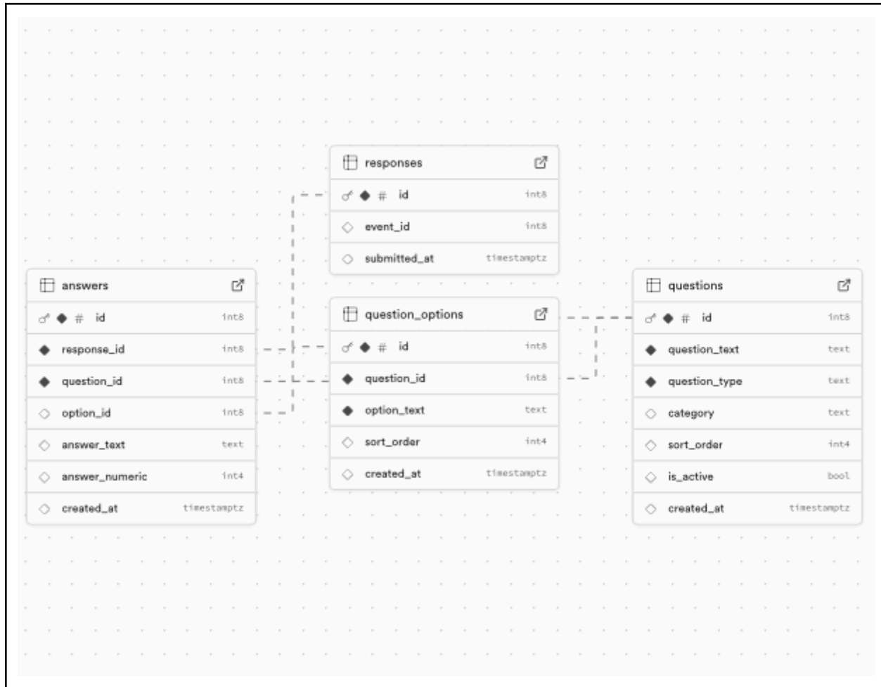
Figure 2: ERD Diagram
