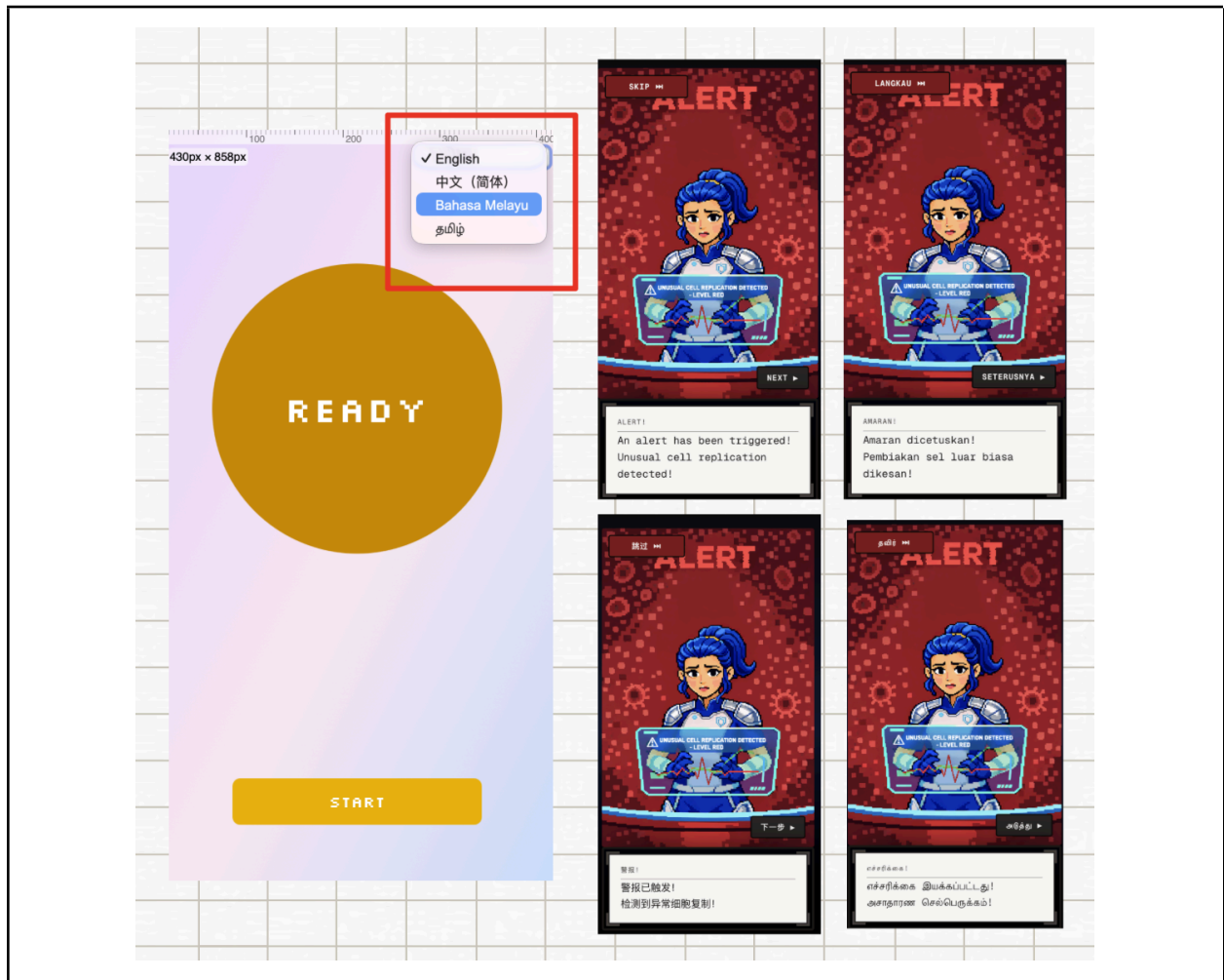
Figure 7: Translation Example
