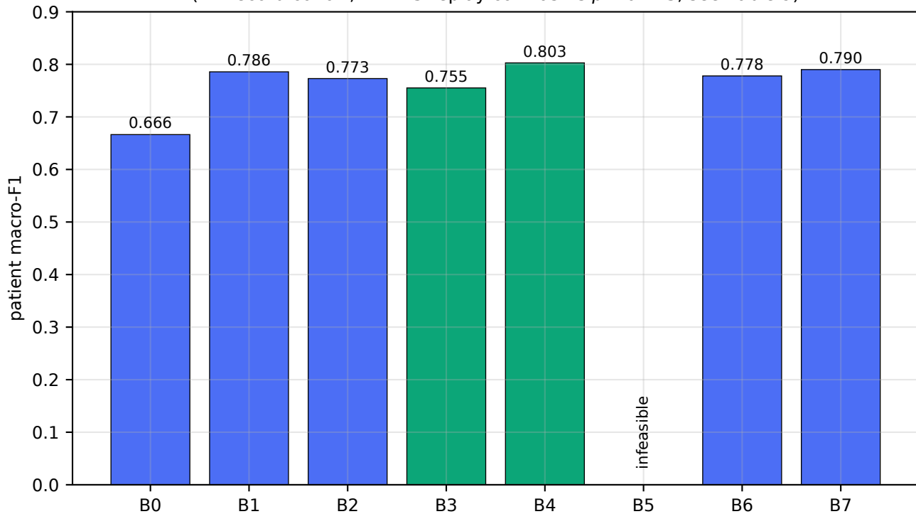
E9 controlled replay-versus-plasticity matrix, arm means only (21-record cohort; B4–B3 replay contrast is p = 0.473 , see Table 9)
