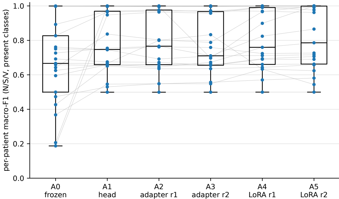
Per-patient adaptation performance (21-record patient-disjoint cohort, 5 seeds averaged per patient)
