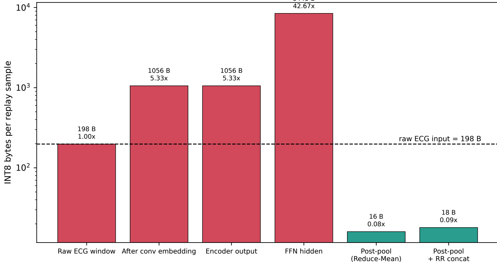
Replay-point cliff in the tiny ECG transformer
