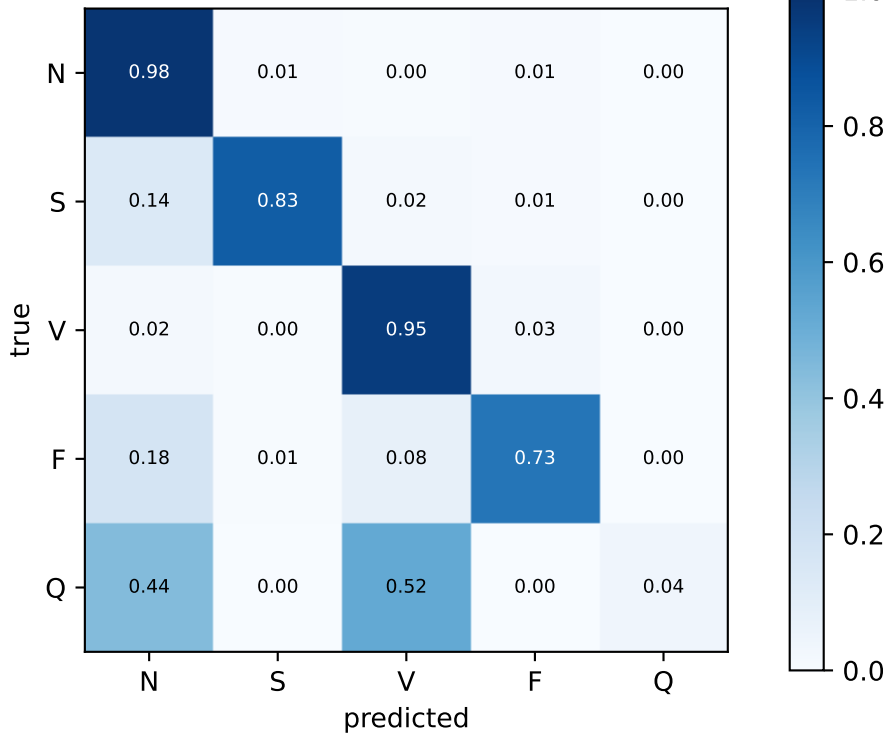
A5 pooled (row-normalized)
