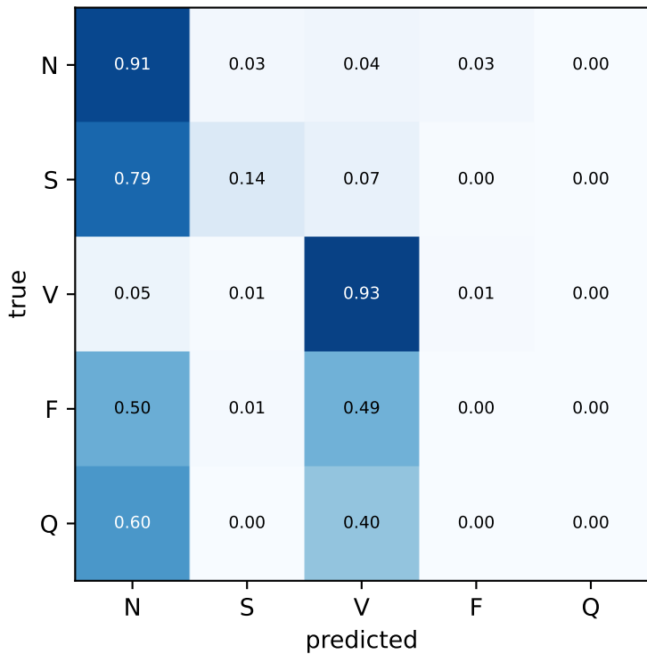
A0 pooled (row-normalized)
