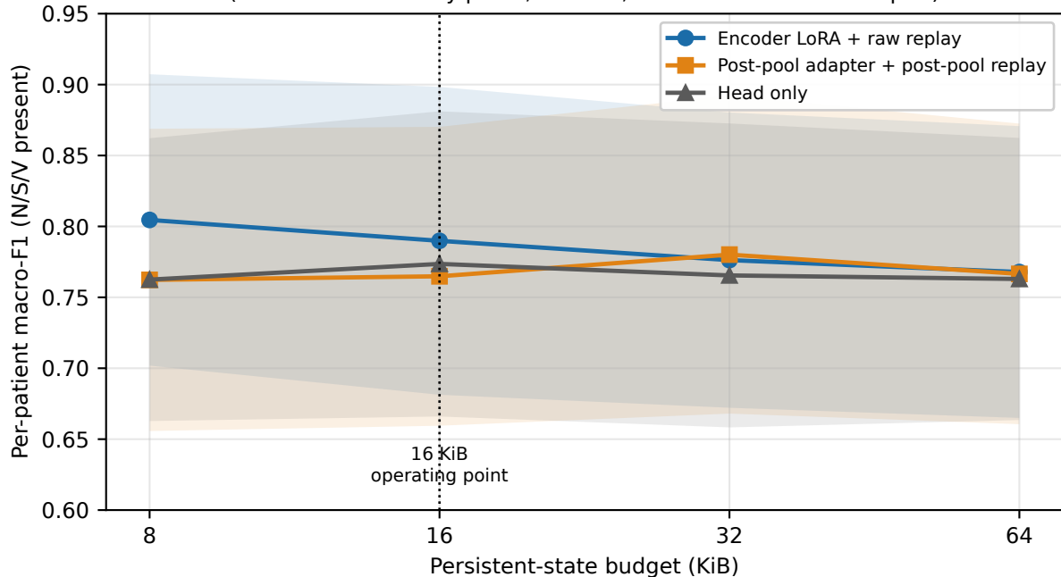
Budget saturation, Adam sweep panel (12-record secondary panel, 3 seeds; shaded = 95% bootstrap CI)
