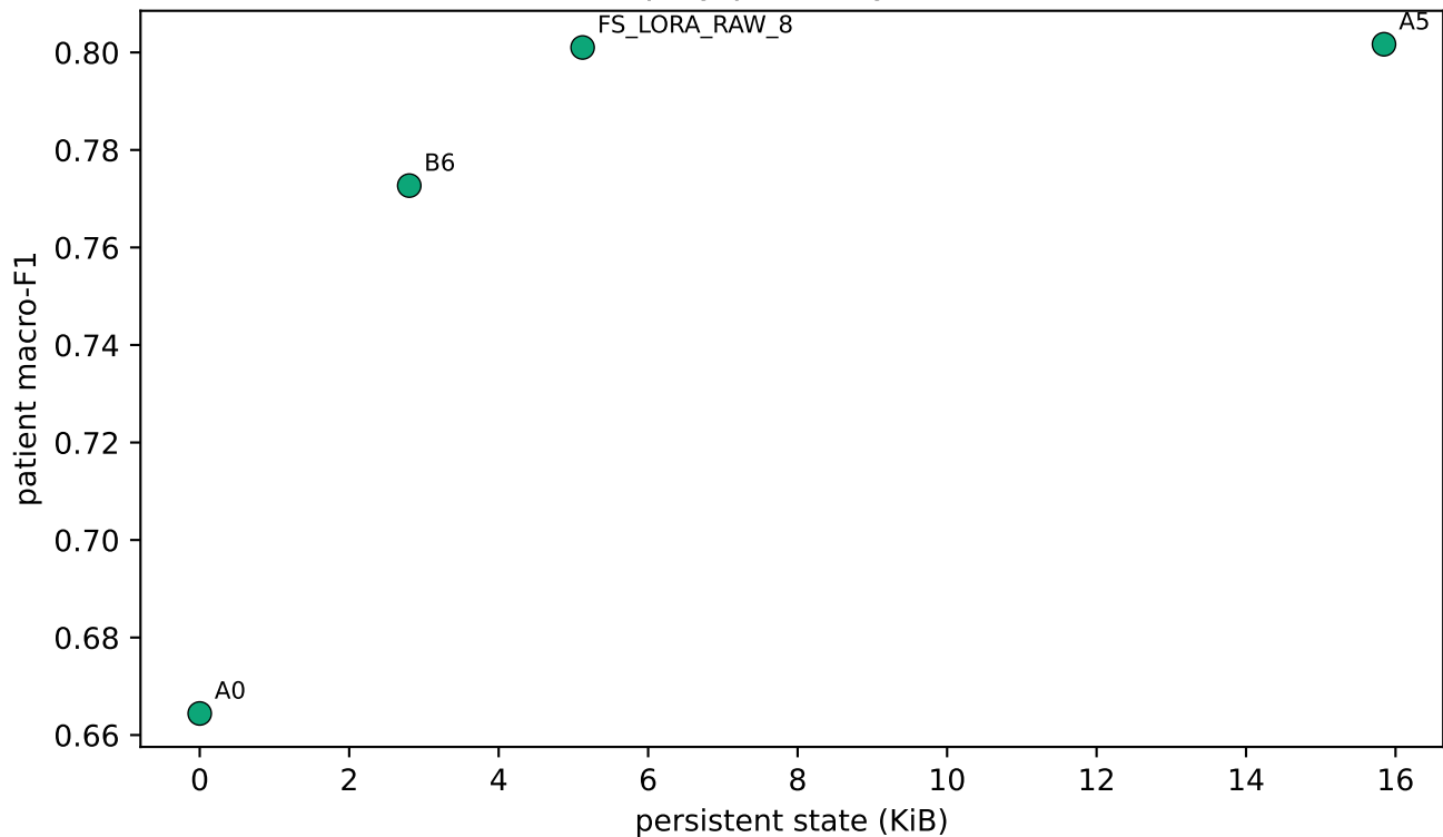
Measured replay-plasticity Pareto frontier
