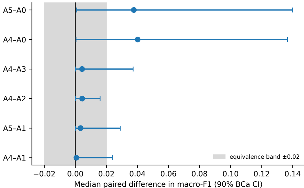
Paired differences vs. pre-registered \pm\delta equivalence band
